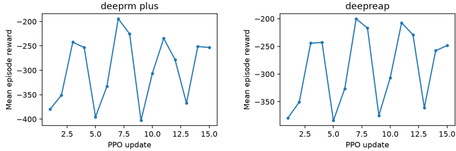
Fig. 5. PPO learning curves for DEEPRM_PLUS (left) and DEEPREAP (right) over 15 updates. Both oscillate without converging; the near-identical trajectories reflect the shared random seed. At this budget PPO refinement degrades both pre-trained policies, so the imitation checkpoint is the one we would deploy.
