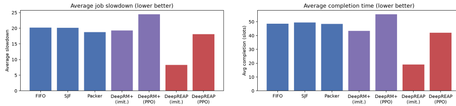
Fig. 4. Average job slowdown (left) and average completion time in slots (right) across all seven schedulers; lower is better in both. DEEPREAP-imitation reaches 8.27 slowdown, less than half the best heuristic result of 18.76, with the completion ordering closely tracking it.
