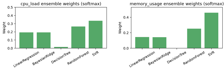
Fig. 3. Softmax( \tau=2 ) ensemble weights for cpu_load (left) and memory_usage (right). Mass concentrates on SVR and Random Forest; the Decision Tree receives near-zero weight.
