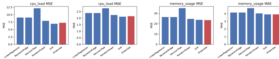
Fig. 2. REAP base-model and softmax-ensemble error, MSE (left panel of each pair) and MAE (right). Left: cpu_load — SVR is lowest; the ensemble is second. Right: memory_usage — the ensemble bar is lowest in both panels.
